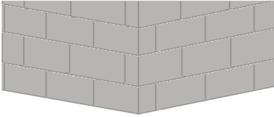
An outside 90 degree mitered corner.
